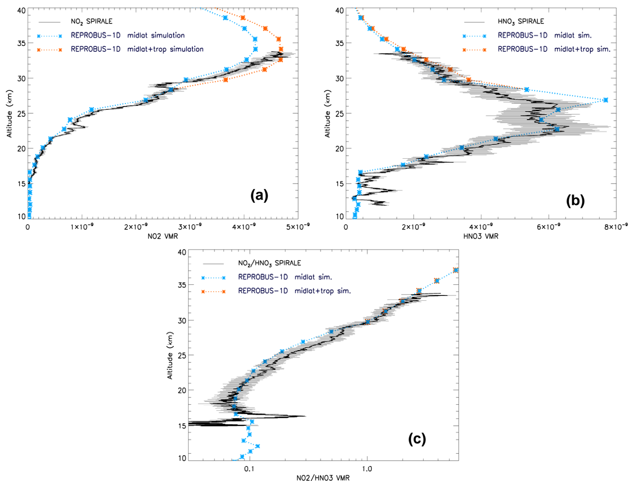
Fig. 10. \text{NO}_2 (a), \text{HNO}_3 (b) and \text{NO}_2/\text{HNO}_3 ratio (c) measured by SPIRALE (black curve) and simulated by Reprobus. The model is here constrained by the measured profile of \text{N}_2\text{O} and the \text{NO}_y^* deduced from the \text{N}_2\text{O} - \text{NO}_y correlation. Blue curve: Reprabus-1-D-midlat experiment, \text{NO}_y^* profile inferred from the correlation valid in the 28–46° N latitude band. Orange curve: Reprabus-1-D-midlat-trop experiment, \text{NO}_y^* profile inferred from the correlation valid in the 3–10° N latitude band, only shown above 29 km where the air seems to mostly originate from low latitudes.
