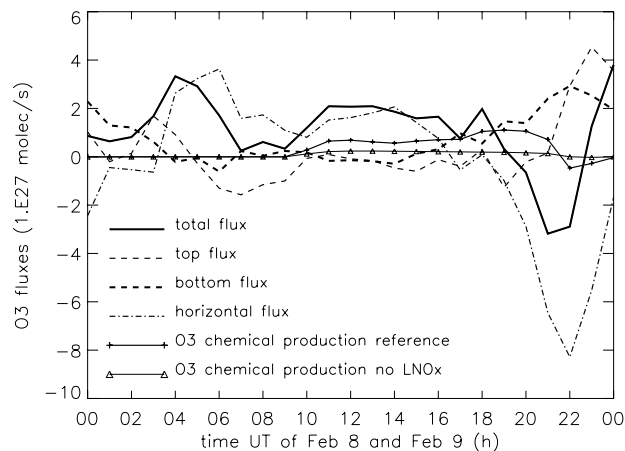
Fig. 8. O_3 instantaneous fluxes on each side of the domain shown in Fig. 7 between 8 February 00:00 UT and 9 February 00:00 UT for the “reference” run. The positive sign of the flux means that the flux is entering the domain. Also shown are the instantaneous O_3 chemical production within the domain for both simulations and the total of each flux including the O_3 production (solid line) for the “reference” run.
