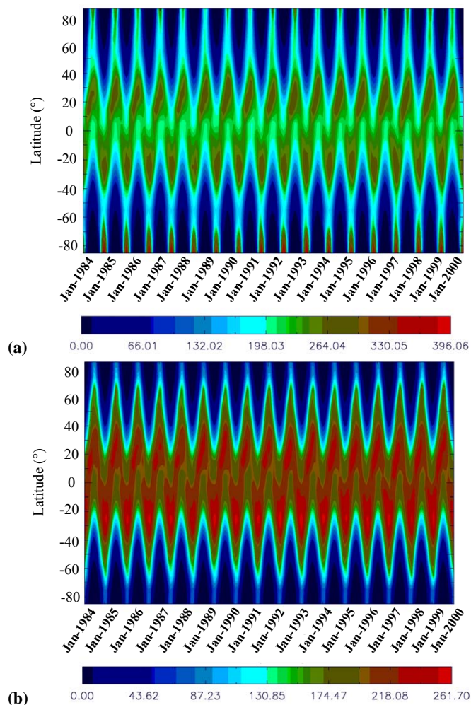
Fig. 4. Time-series of 10-degree latitude-zonal averages of monthly mean (a) downward shortwave radiation (DSR) at the Earth's surface and (b) net downward shortwave radiation (Net DSR) at the Earth's surface, for the period January 1984 – December 2000. Monthly mean quantities over a 2.5^{\circ} \times 2.5^{\circ} geographical grid are used.
