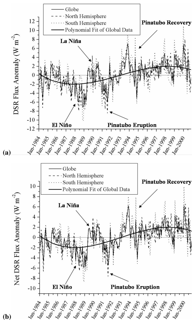
Fig. 6. Time-series of global and hemispherical averages of (a) downward shortwave radiation (DSR) flux anomalies (in \text{Wm}^{-2} ) and (b) net downward shortwave radiation (DSR) flux anomalies (in \text{Wm}^{-2} ) over the period 1984–2000 for the Globe (solid lines), Northern Hemisphere (dashed lines), and Southern Hemisphere (dotted lines). The 4th-order polynomial fit of the global data is also shown.
