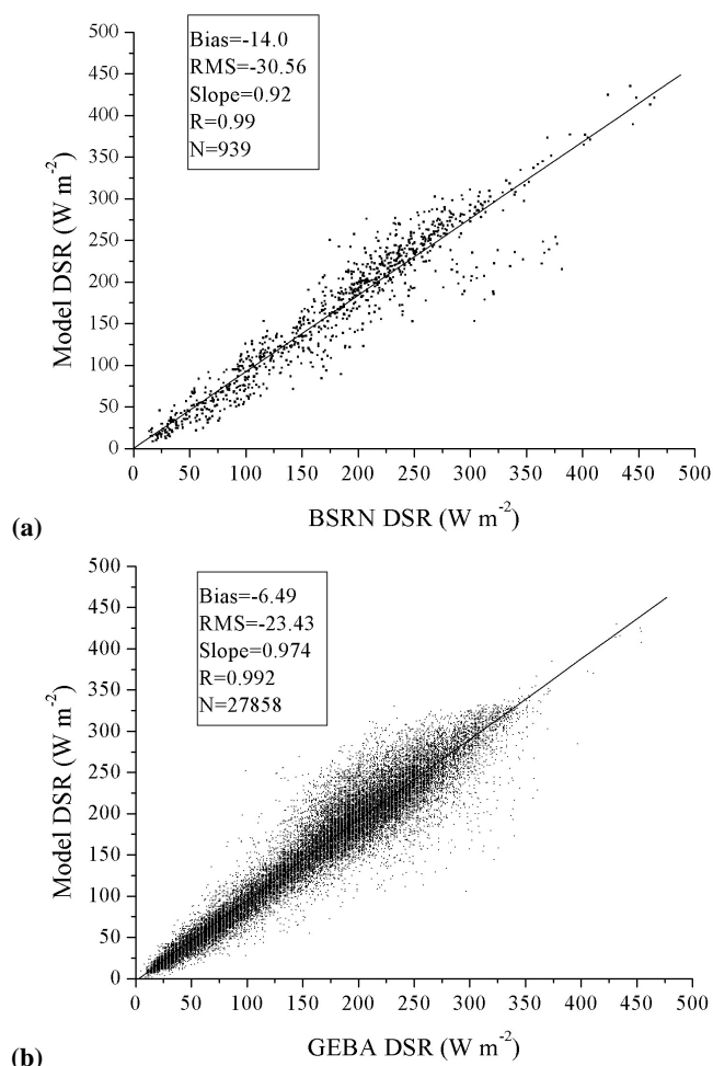
Fig. 9. Scatter plot comparison between model-computed and: (a) Baseline Surface Radiation Network (BSRN), and (b) Global Energy Balance Archive (GEBA) grid-cell data of monthly average downward shortwave radiation (DSR) at the Earth's surface, over the time periods 1992–2000 and 1984–2000, respectively. R and N are the correlation coefficient and number of matched data pairs, respectively.
