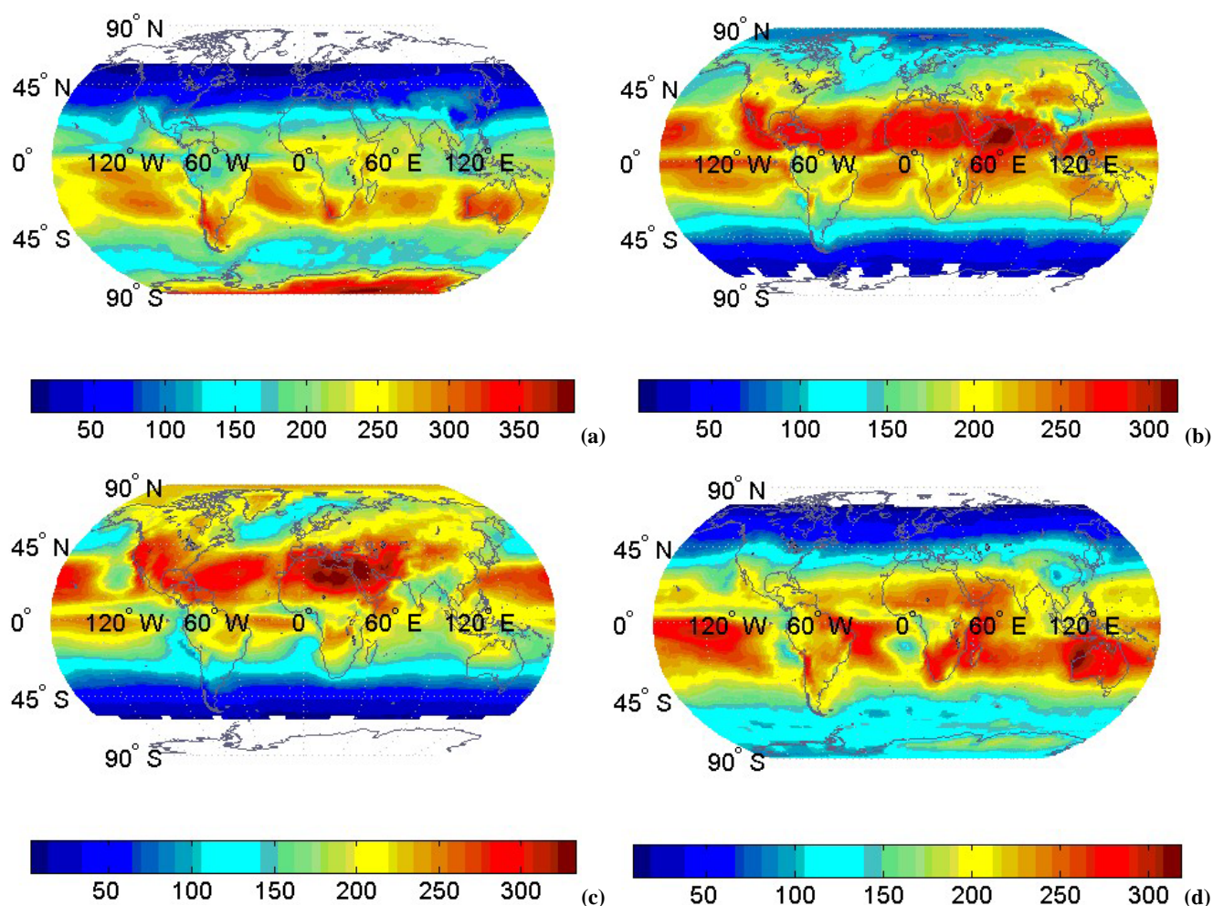
Fig. 1. Long-term (1984–2000) average global distribution of downward shortwave radiation (in \text{Wm}^{-2} ) at the Earth's surface for the mid-seasonal months of (a) January, (b) April, (c) July, and (d) October.
