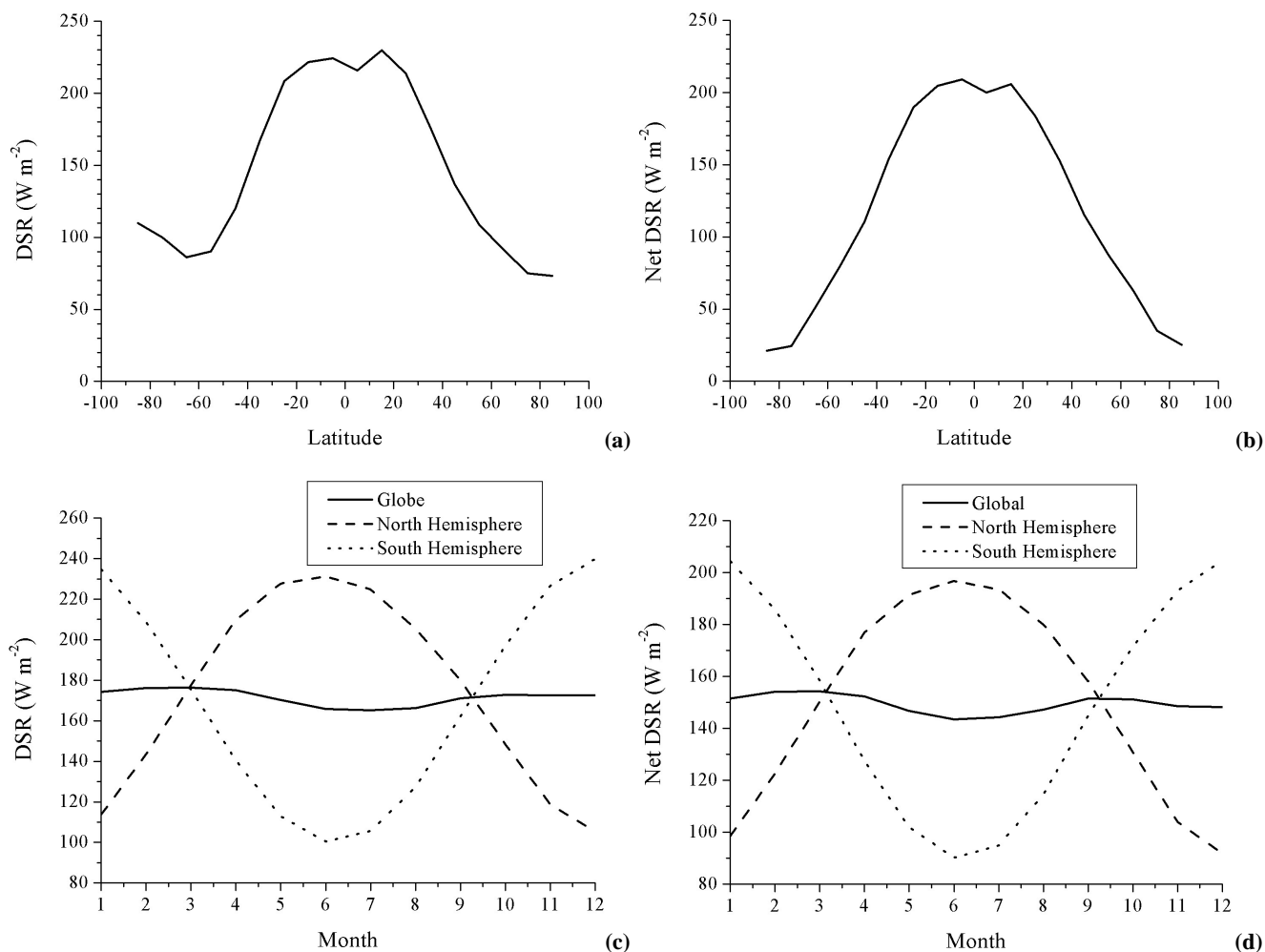
Fig. 7. Latitudinal variation of model computed: (a) mean annual downward shortwave radiation (DSR in \text{W m}^{-2} ) at the Earth's surface, and (b) mean annual net downward (or absorbed) shortwave radiation (Net DSR in \text{W m}^{-2} ) at the Earth's surface, averaged over the period January 1984 through December 2000. Also shown is the seasonal variation of hemispherical and global averages of model computed: (c) downward shortwave radiation (DSR in \text{W m}^{-2} ) at the Earth's surface, and (d) net downward (or absorbed) shortwave radiation (Net DSR in \text{W m}^{-2} ) at the Earth's surface, averaged over the period January 1984 through December 2000.
