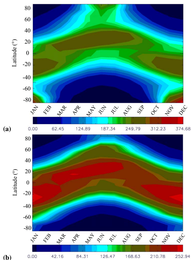
Fig. 3. Seasonal and latitudinal variation of 17-year (1984–2000) averages of monthly mean (a) downward shortwave radiation (DSR) at the Earth's surface and (b) net downward shortwave radiation (Net DSR) at the Earth's surface. Monthly mean quantities over a 2.5^{\circ} \times 2.5^{\circ} geographical grid are plotted.
