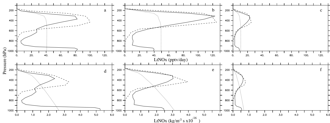
Fig. 2. Monthly mean LtNO x emissions, from model output, in pptv/day (a–c) and 10 −16 kg/m 3 s (d–f), for the three vertical distributions in this study: PICK (solid line), ANVIL (dashed line) and EVEN (dotted line), at selected locations representative of the PICK distribution’s three cases: (a) and (d) midlatitude continental (35° N, 90° W for June 97); (b) and (e) tropical continental (8° N, 65° W for July 1997) and (c) and (f) tropical marine (12° N, 63° W for July 1997).
