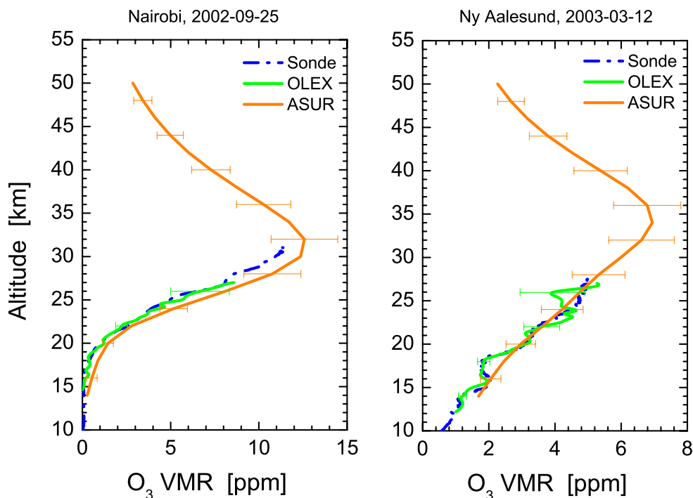
Fig. 9. ASUR, OLEX, and sonde O_3 profiles. Ozone sondes were launched in Nairobi ( 1.27^\circ S, 36.80^\circ E) at 07:23 UT and in Ny Ålesund ( 78.93^\circ N, 11.95^\circ E) at 10:54 UT. Corresponding ASUR measurements including error bars are at 06:52 UT ( 0.61^\circ S, 34.60^\circ E) and at 09:28 UT ( 78.83^\circ N, 12.42^\circ E), respectively. OLEX and ASUR profiles were recorded within a time difference of less than 10 min. The integration time was 5 and 2 min, respectively.
