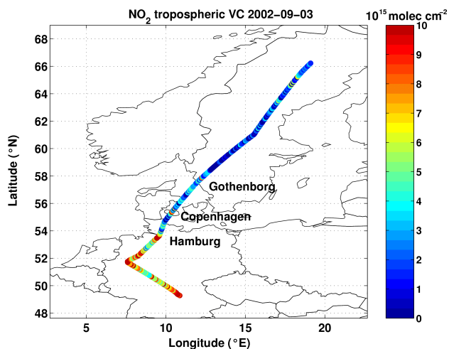
Fig. 7. AMAXDOAS tropospheric \text{NO}_2 vertical columns along the flight track on 3 September 2002 from Oberpfaffenhofen to Kiruna. Enhanced \text{NO}_2 columns were observed in regions affected by tropospheric pollution.
