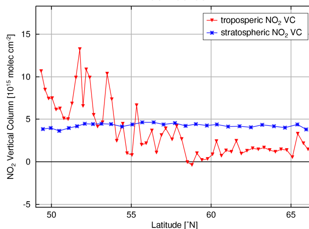
Fig. 8. AMAXDOAS vertical \text{NO}_2 columns for the stratosphere (blue) and troposphere (red) for the same flight as for Fig. 7. The stratospheric \text{NO}_2 did not change much during the flight, whereas in the troposphere pollution leads to strongly varying columns.
