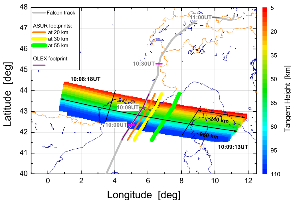
Fig. 4. The panel gives an indication of the footprints of OLEX and ASUR in relation to the SCIAMACHY limb measurements. On 28 September 2002, the Falcon crossed a SCIAMACHY pixel (Orbit No. 3025, state index 12) near Marseille, France, in northerly direction (gray line with time markers). At each tangent height of the SCIAMACHY measurement (height step = 3 km) the total swath of 960 km is divided into 4 separate measurements (read-outs) of \sim 240 km width. Details on the viewing geometry of SCIAMACHY can be found in (Bovensmann et al., 1999).
