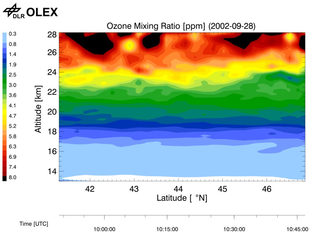
Fig. 11. OLEX measurement of the ozone distribution on the measurement flight on 28 September 2002. The Falcon flight pattern is given in Fig. 4. The overpass of SCIAMACHY took place at 10:09 UTC around 43° N.
