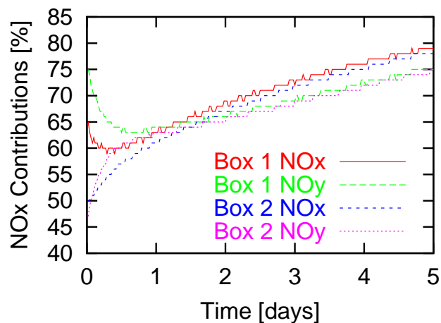
Fig. 1. Temporal development of the \text{NO}_x and \text{NO}_y contributions (%) from a \text{NO}_x source simulated with a two-box model with characteristics of a GCM simulation representing mid latitudes at 300 hPa (see text and appendix for details).
