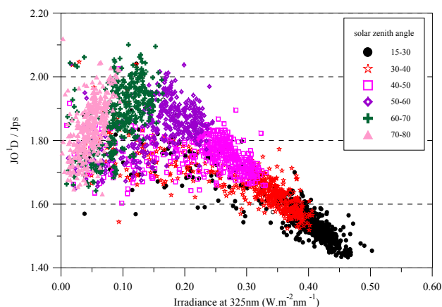
Fig. 6. Ratio of J(O 1 D)/ Jps , as a function of global irradiance at 325 nm for different groups of solar zenith angles. (J(O 1 D)) was calculated from the spectral actinic flux data from the Bentham spectroradiometer and Jps is calculated if the global irradiance is used instead of actinic flux in Eq. 1).
